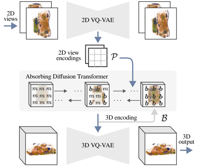
Figure 1. The proposed approach independently learns a discrete information-rich codebook for 2D and 3D domains with two VQ-VAEs. New 3D samples are then synthesized conditional on the complete codebook of multiple 2D views with a transformer.
